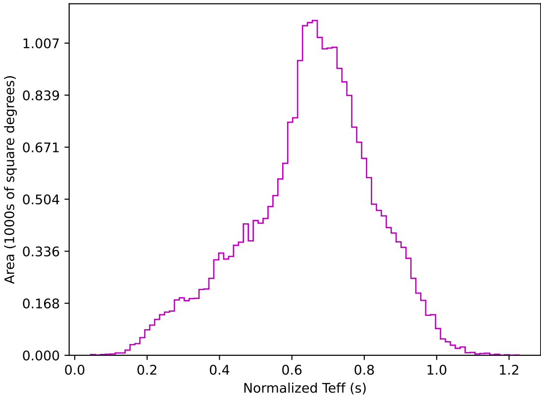
ddf_acor_sf10_lsf30_lsr10_v3.4_10yrs All sky z band: Normalized Teff
