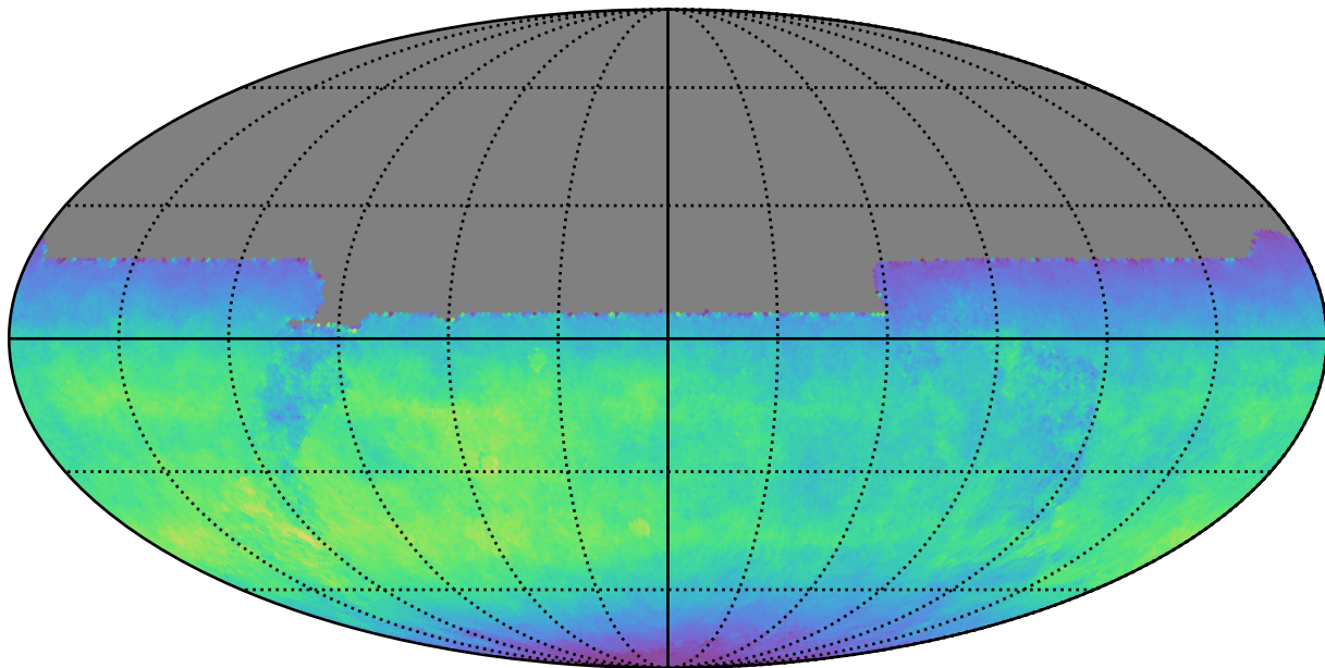
ddf_acor_sf10_lsf30_lsr10_v3.4_10yrs All sky y band: Normalized Teff
