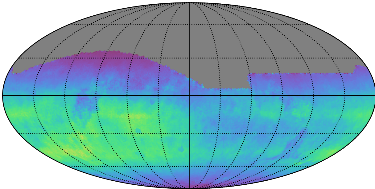
ddf_acor_sf10_lsf30_lsr10_v3.4_10yrs All sky r band: Normalized Teff
