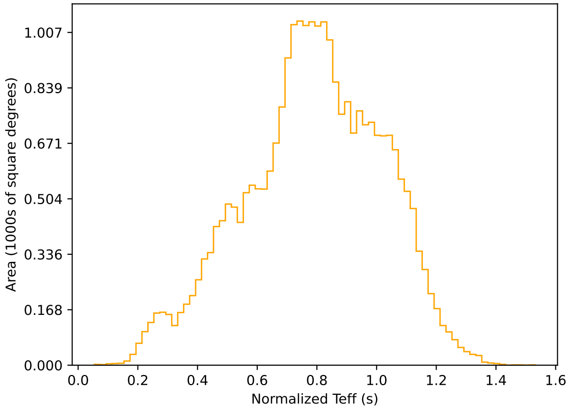
ddf_acor_sf10_lsf30_lsr10_v3.4_10yrs All sky r band: Normalized Teff
