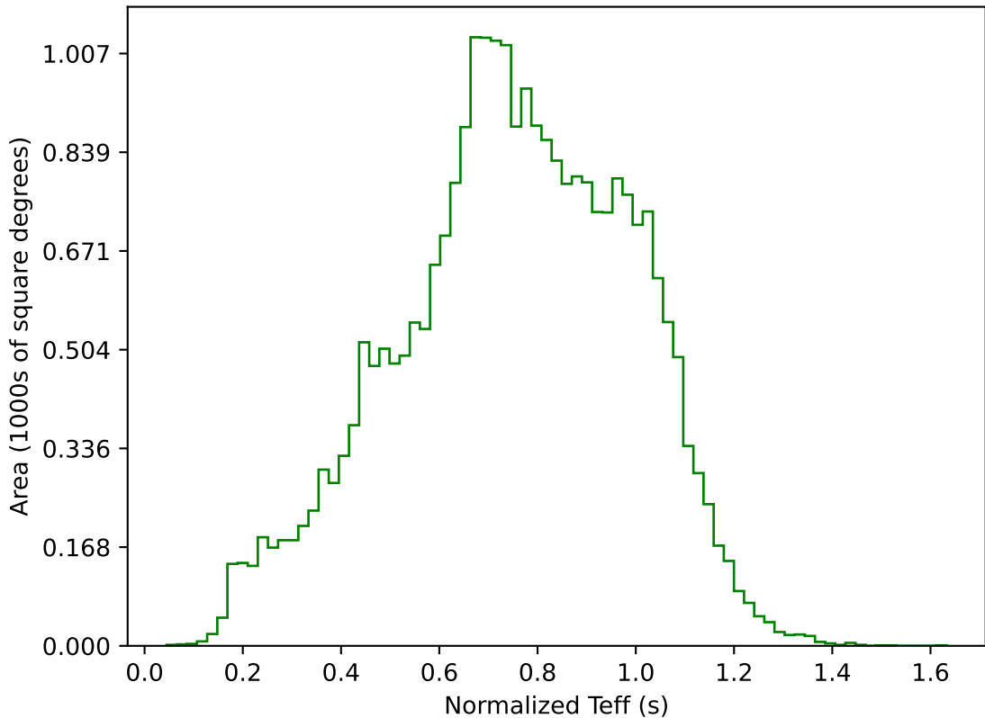
ddf_acor_sf10_lsf30_lsr10_v3.4_10yrs All sky g band: Normalized Teff
