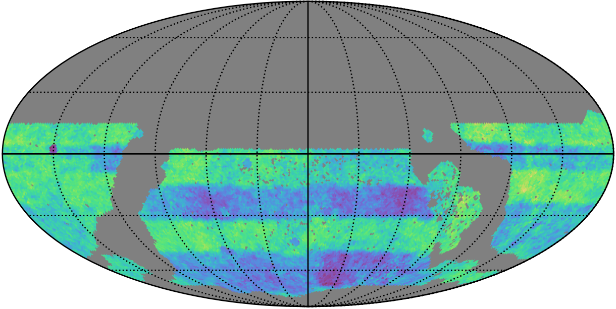
ddf_acor_sf10_lsf30_lsr10_v3.4_10yrs WFD: Normalized Proper Motion Uncert @ 24.0
