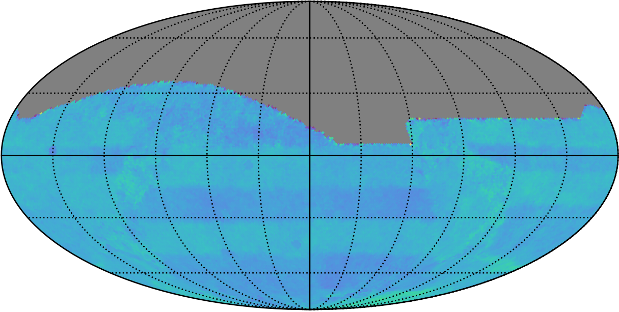
ddf_acor_sf10_lsf30_lsr10_v3.4_10yrs All sky: Normalized Proper Motion Uncert @ 24.0
