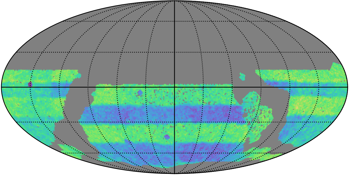
ddf_acor_sf10_lsf30_lsr10_v3.4_10yrs WFD: Normalized Proper Motion Uncert @ 20.5
