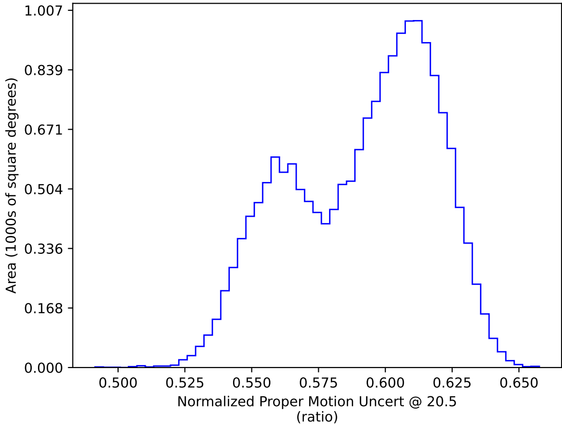
ddf_acor_sf10_lsf30_lsr10_v3.4_10yrs WFD: Normalized Proper Motion Uncert @ 20.5
