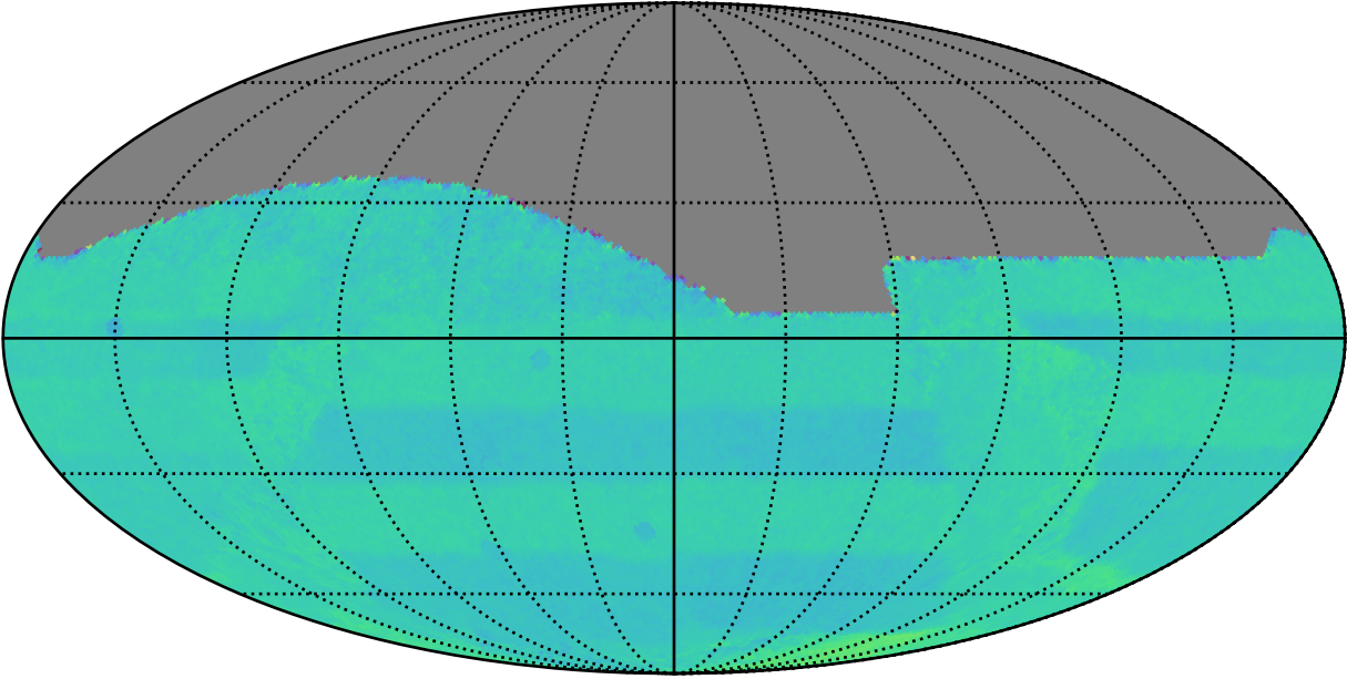
ddf_acor_sf10_lsf30_lsr10_v3.4_10yrs All sky: Normalized Proper Motion Uncert @ 20.5
