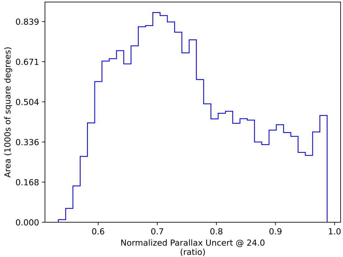
ddf_acor_sf10_lsf30_lsr10_v3.4_10yrs WFD: Normalized Parallax Uncert @ 24.0
