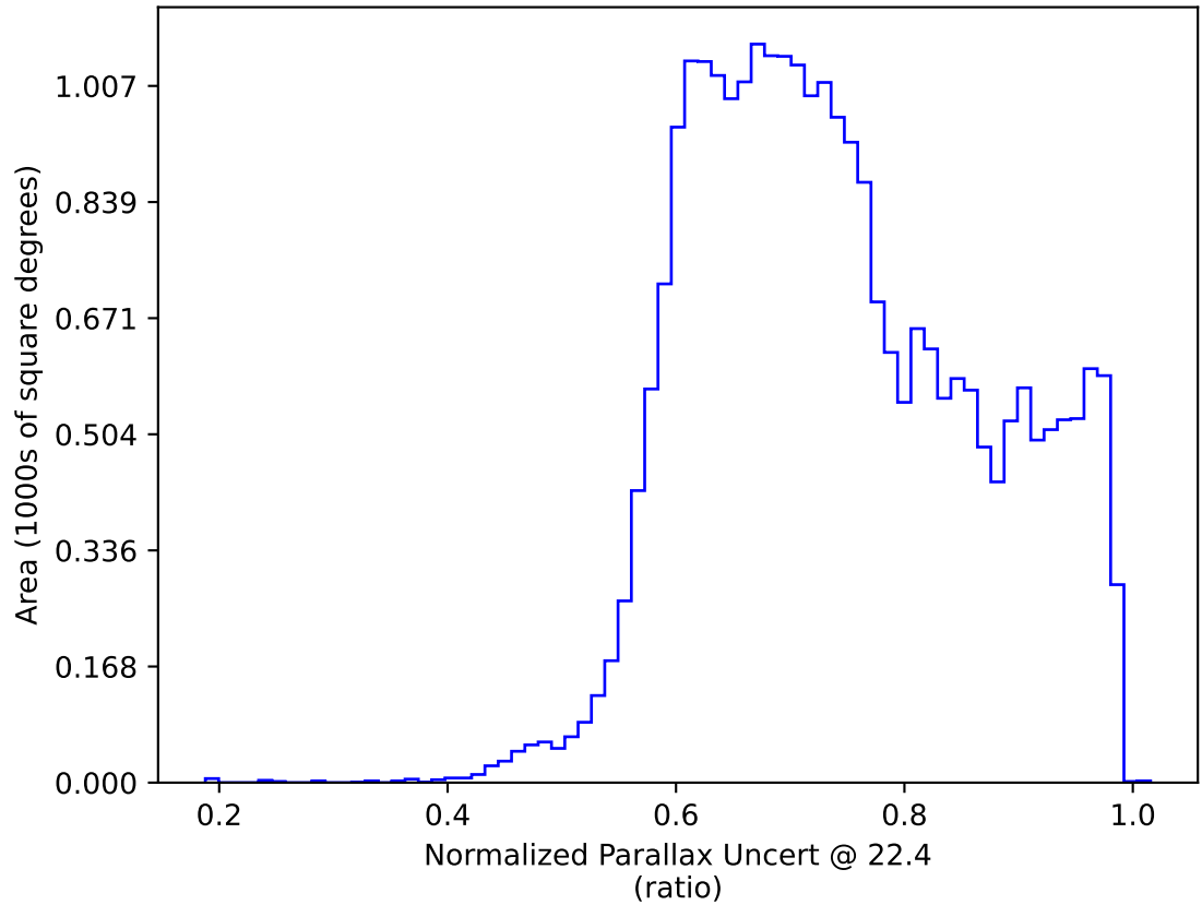
ddf_acor_sf10_lsf30_lsr10_v3.4_10yrs All sky: Normalized Parallax Uncert @ 22.4
