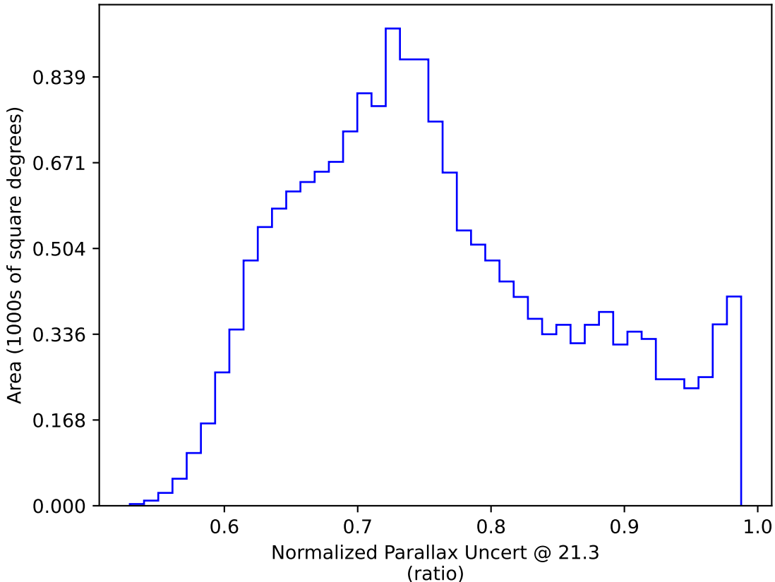
ddf_acor_sf10_lsf30_lsr10_v3.4_10yrs WFD y band only: Normalized Parallax Uncert @ 21.3
