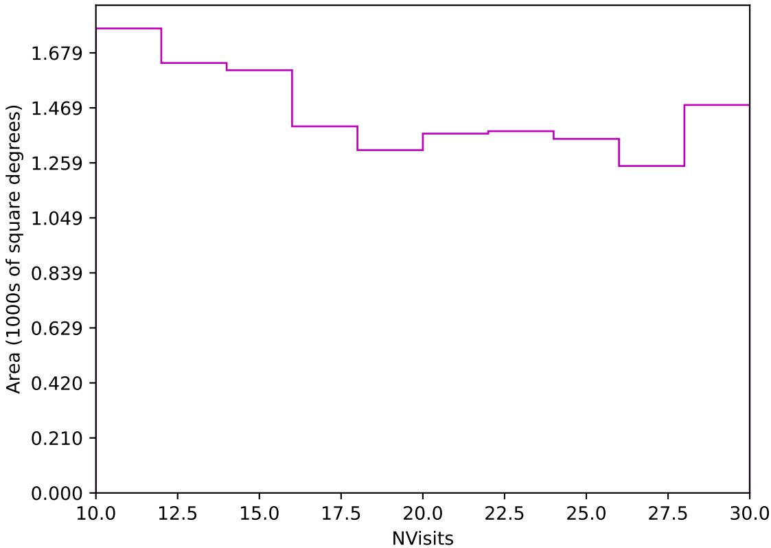
ddf_acor_sf10_lsf30_lsr10_v3.4_10yrs Yr 3-4 z band: NVisits
