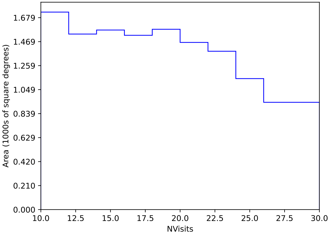
ddf_acor_sf10_lsf30_lsr10_v3.4_10yrs Yr 3-4 y band: NVisits
