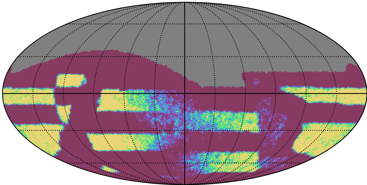
ddf_acor_sf10_lsf30_lsr10_v3.4_10yrs Yr 3-4 all bands: NVisits
