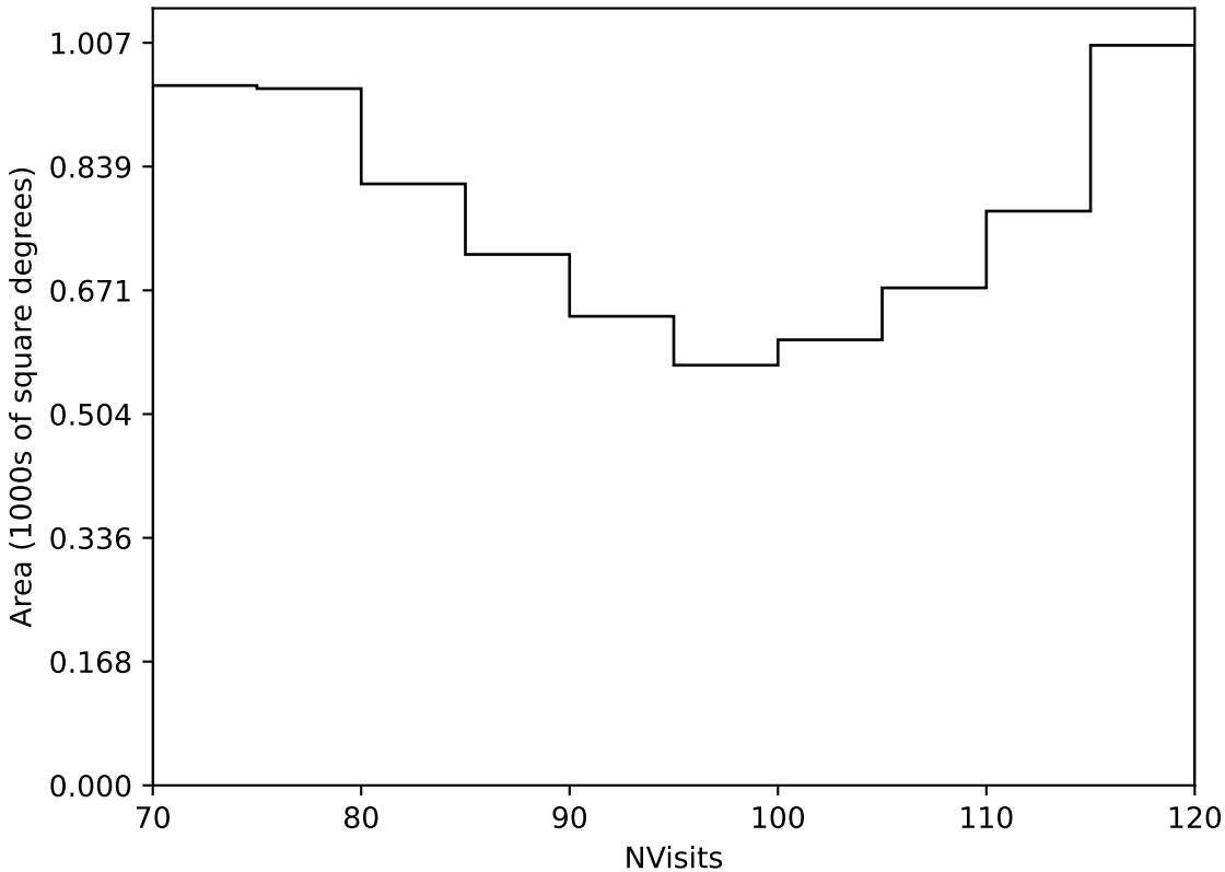
ddf_acor_sf10_lsf30_lsr10_v3.4_10yrs Yr 3-4 all bands: NVisits
