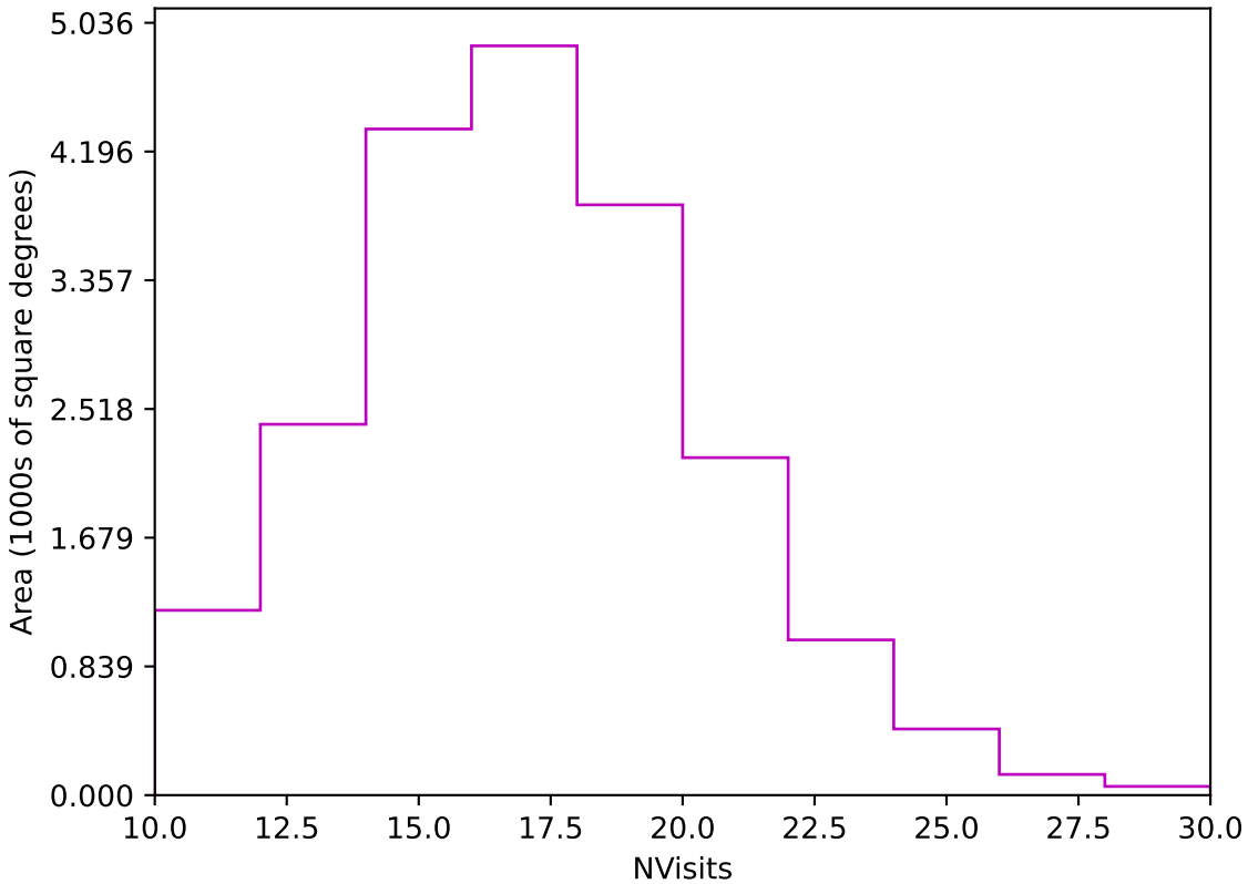
ddf_acor_sf10_lsf30_lsr10_v3.4_10yrs Yr 1 z band: NVisits
