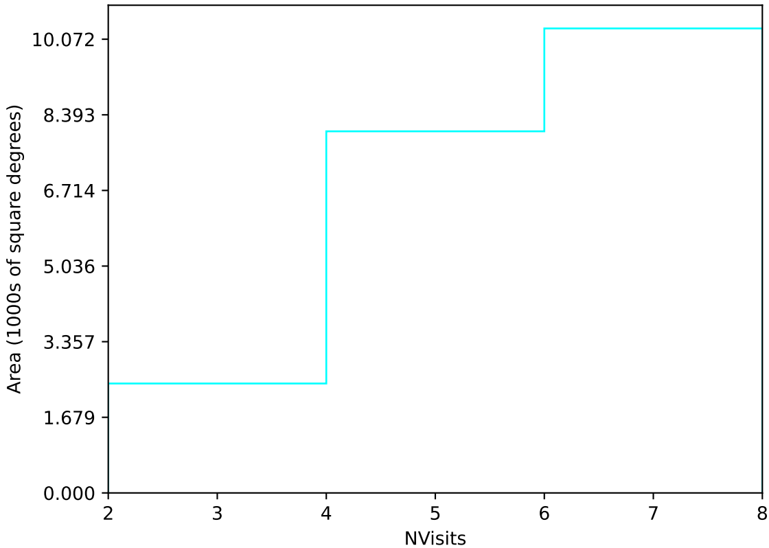
ddf_acor_sf10_lsf30_lsr10_v3.4_10yrs Yr 1 u band: NVisits
