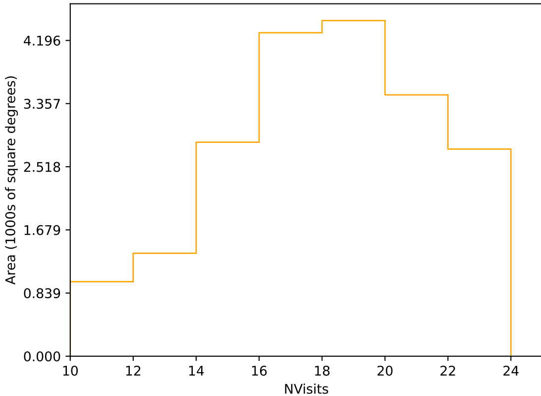
ddf_acor_sf10_lsf30_lsr10_v3.4_10yrs Yr 1 r band: NVisits
