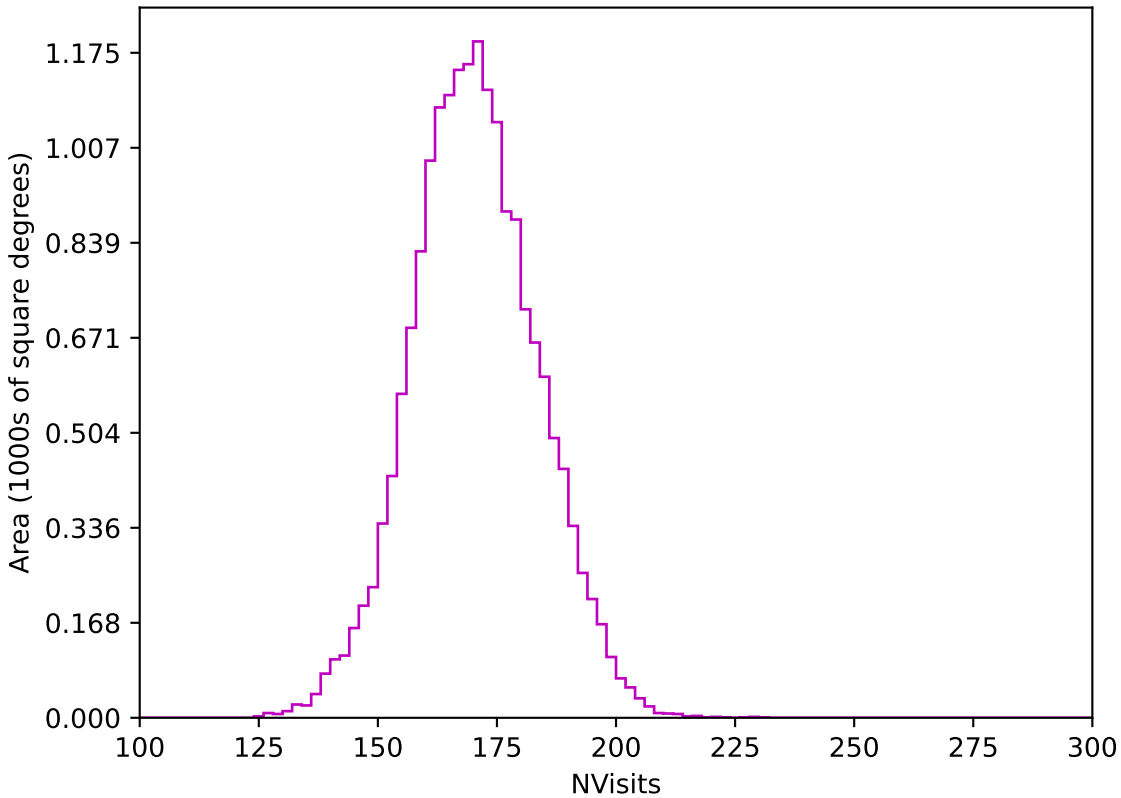
ddf_acor_sf10_lsf30_lsr10_v3.4_10yrs WFD z band: NVisits
