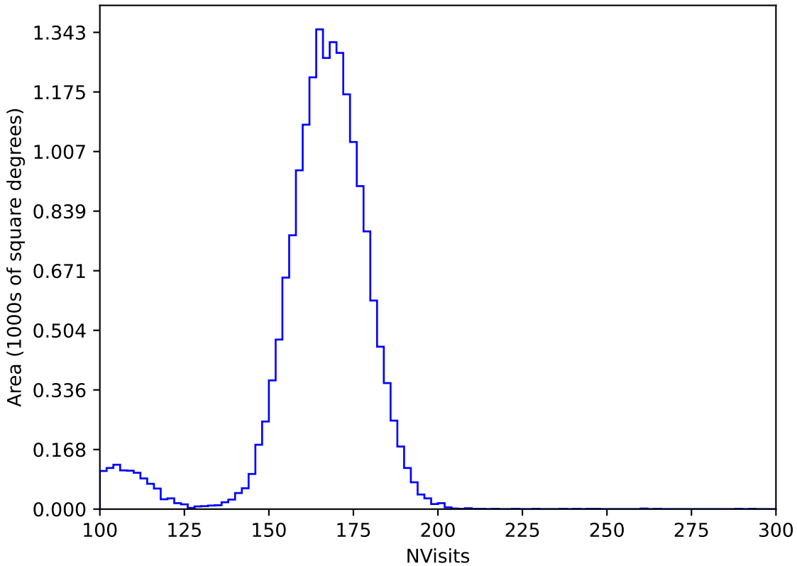
ddf_acor_sf10_lsf30_lsr10_v3.4_10yrs WFD y band: NVisits
