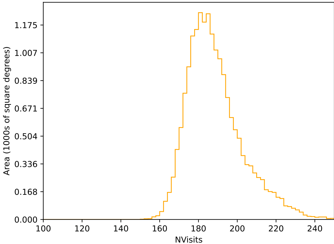
ddf_acor_sf10_lsf30_lsr10_v3.4_10yrs WFD r band: NVisits
