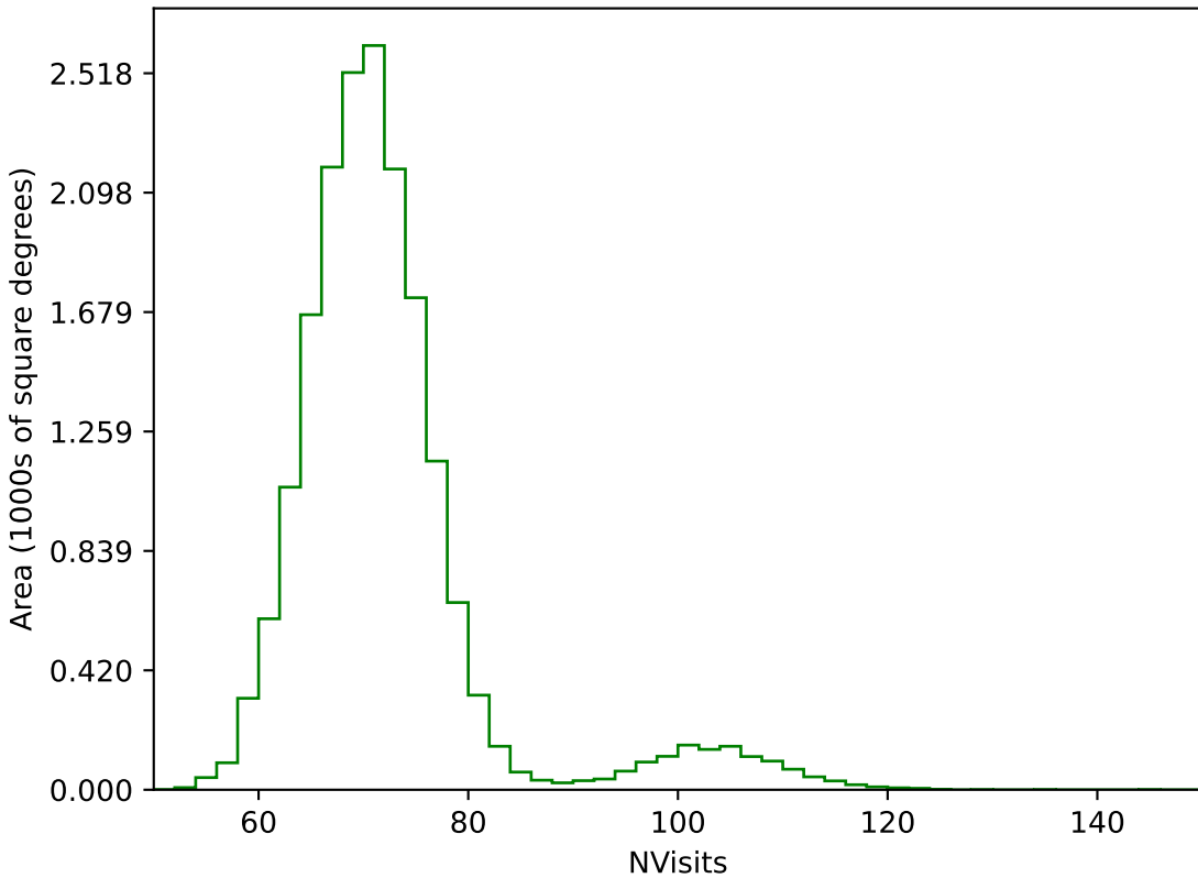
ddf_acor_sf10_lsf30_lsr10_v3.4_10yrs WFD g band: NVisits
