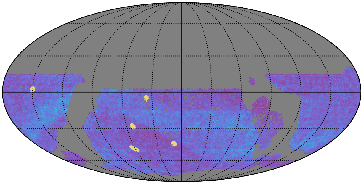
ddf_acor_sf10_lsf30_lsr10_v3.4_10yrs WFD all bands: NVisits
