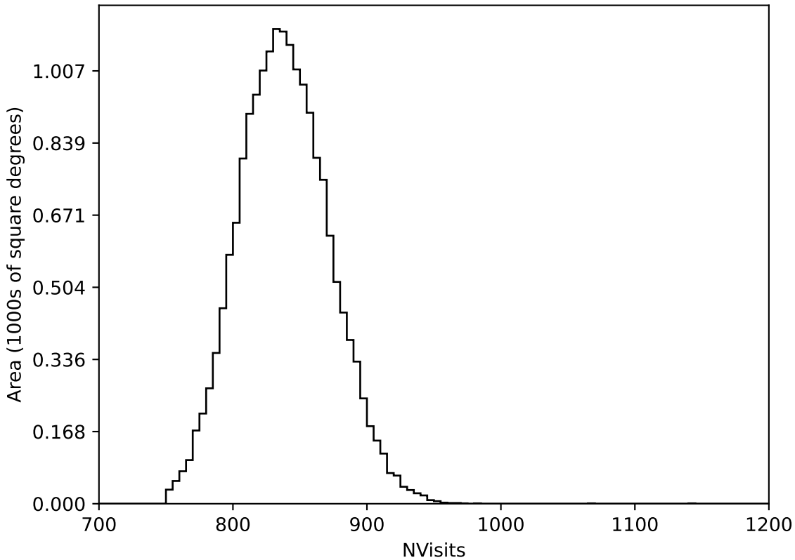
ddf_acor_sf10_lsf30_lsr10_v3.4_10yrs WFD all bands: NVisits
