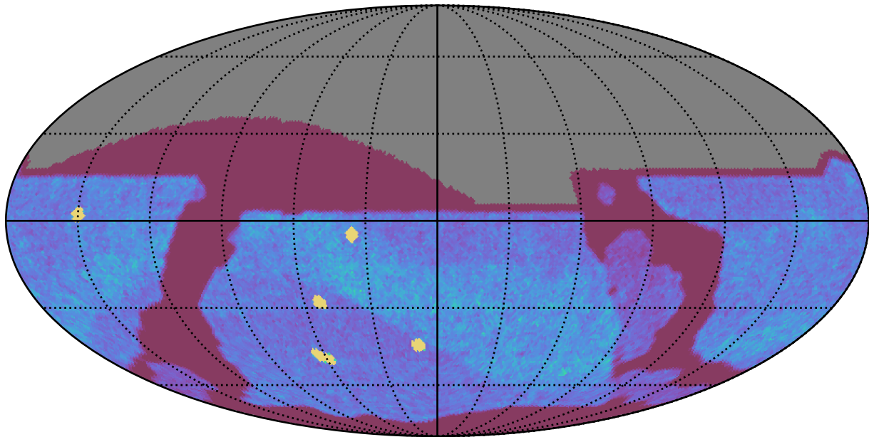
ddf_acor_sf10_lsf30_lsr10_v3.4_10yrs All sky z band: NVisits
