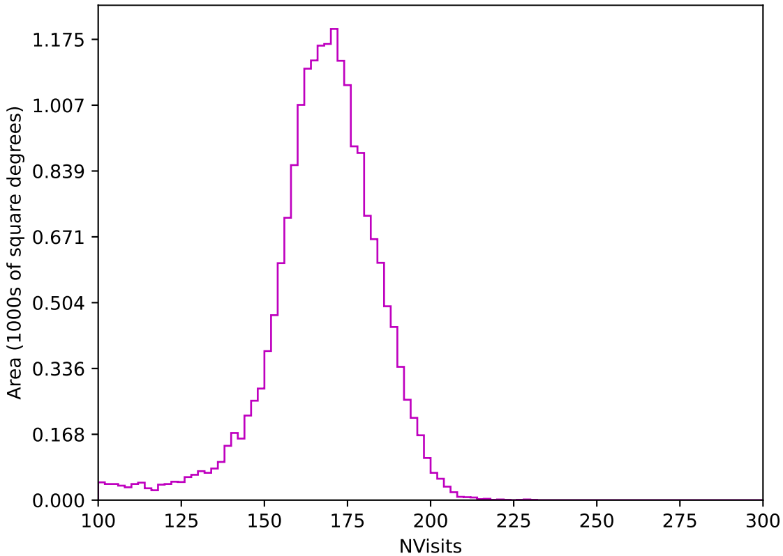
ddf_acor_sf10_lsf30_lsr10_v3.4_10yrs All sky z band: NVisits
