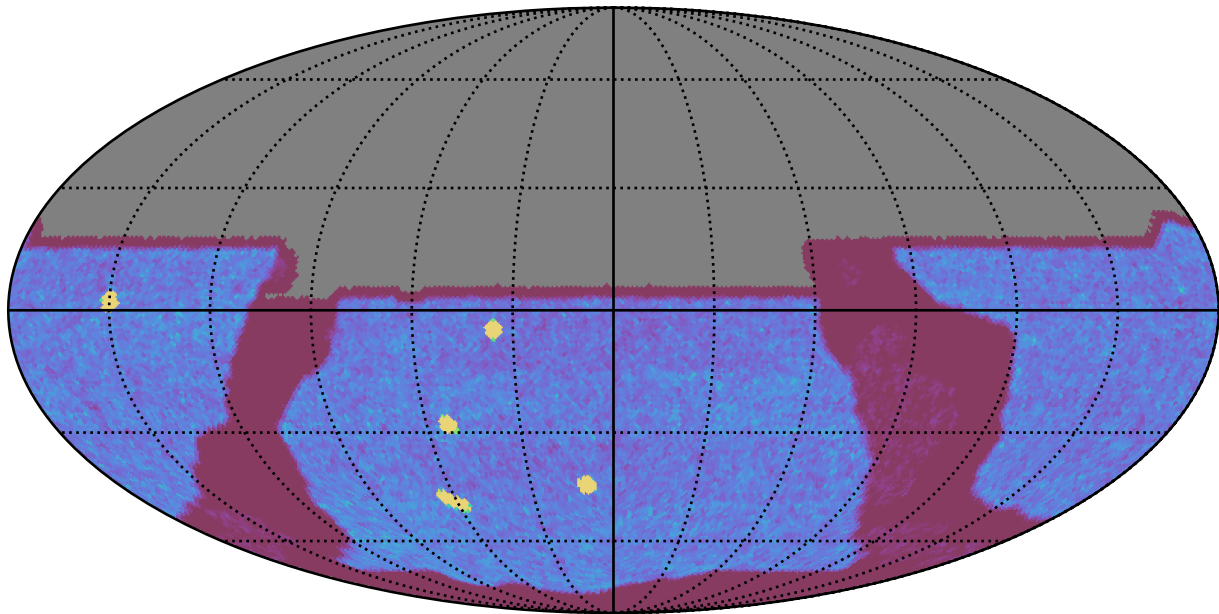
ddf_acor_sf10_lsf30_lsr10_v3.4_10yrs All sky y band: NVisits
