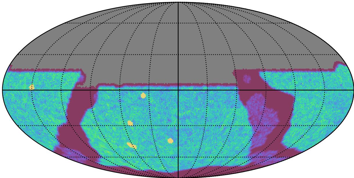
ddf_acor_sf10_lsf30_lsr10_v3.4_10yrs All sky u band: NVisits
