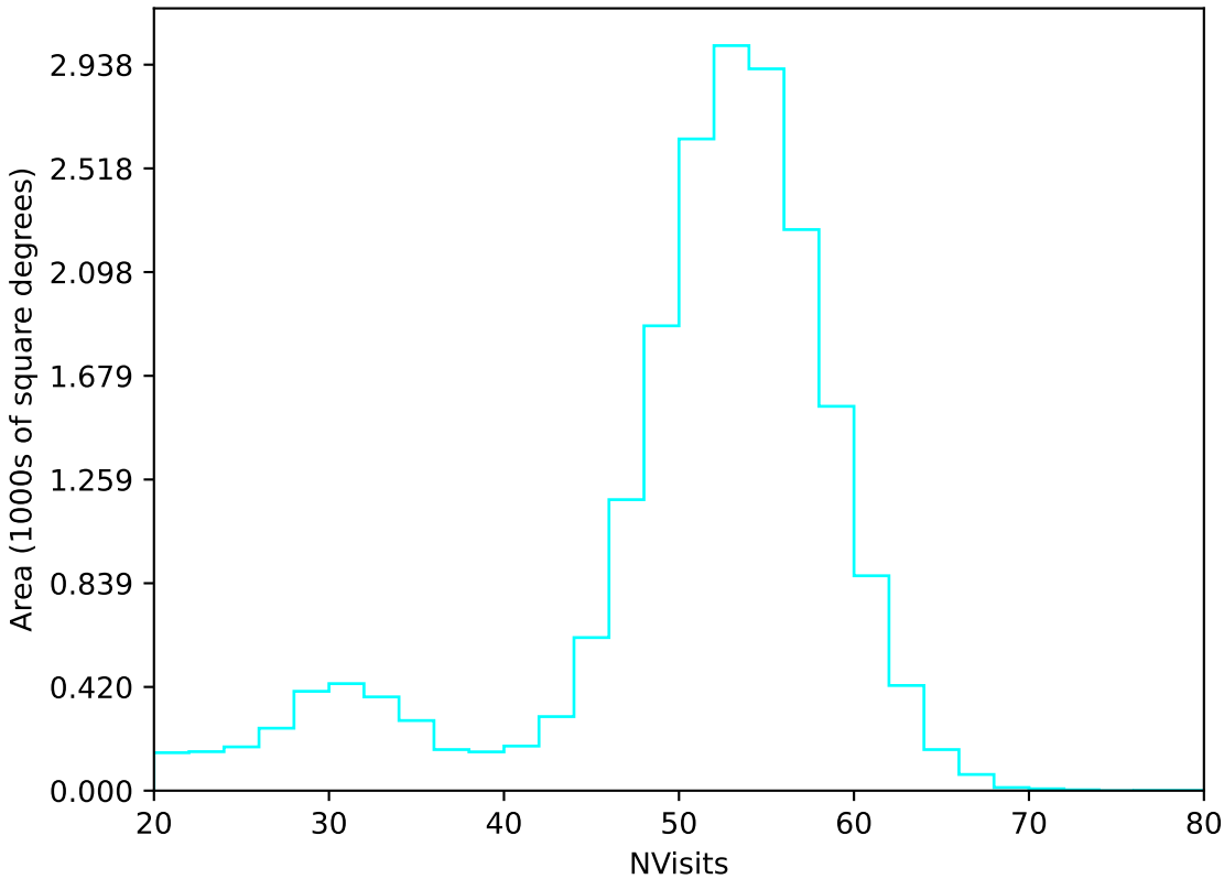
ddf_acor_sf10_lsf30_lsr10_v3.4_10yrs All sky u band: NVisits
