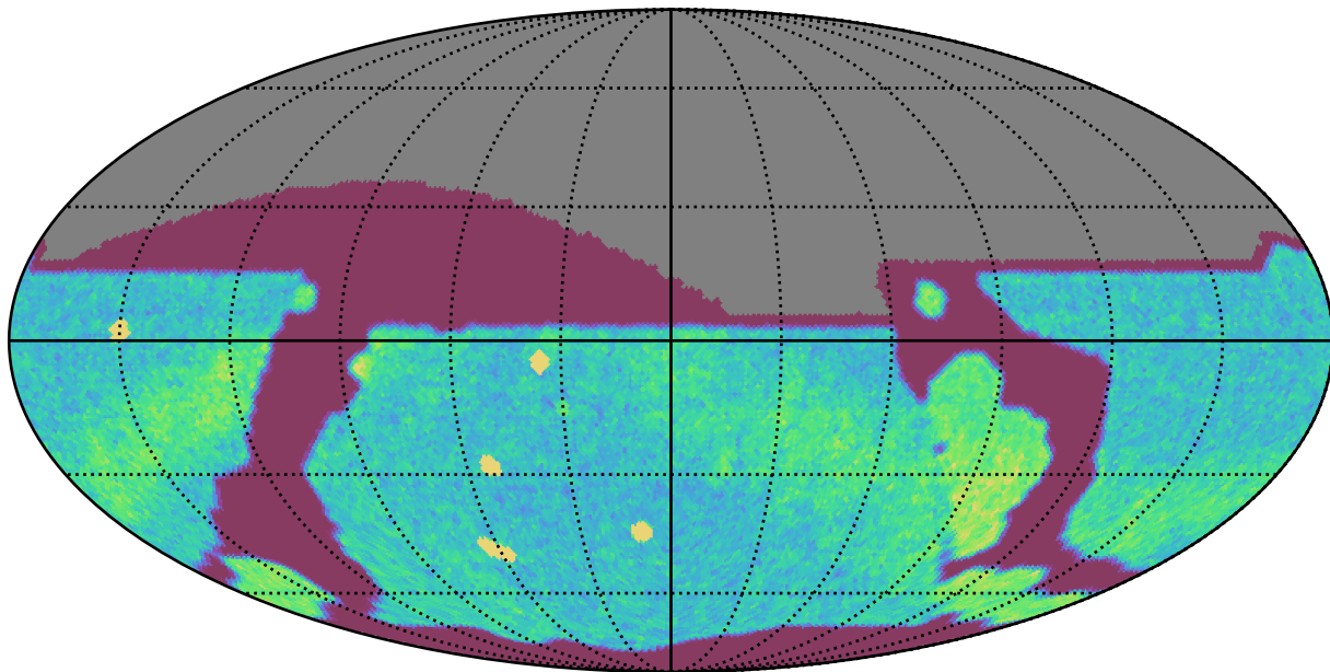
ddf_acor_sf10_lsf30_lsr10_v3.4_10yrs All sky r band: NVisits
