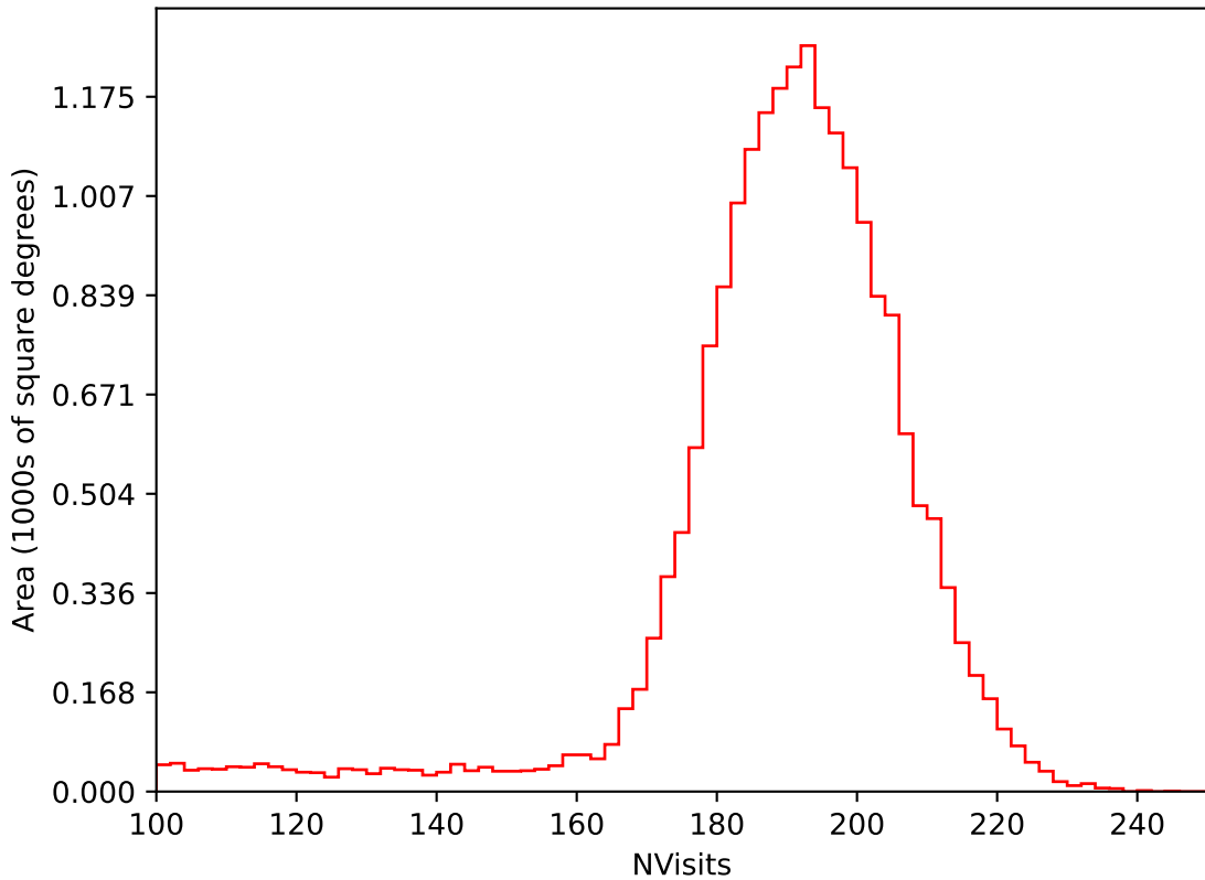
ddf_acor_sf10_lsf30_lsr10_v3.4_10yrs All sky i band: NVisits
