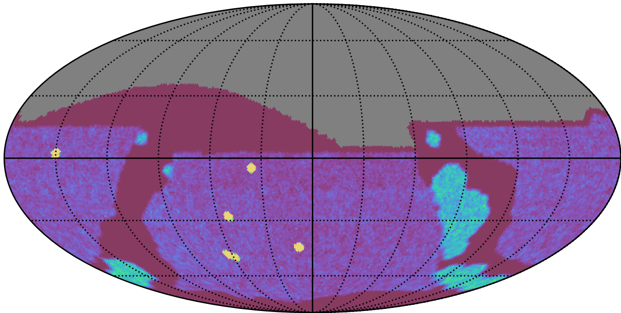
ddf_acor_sf10_lsf30_lsr10_v3.4_10yrs All sky g band: NVisits
