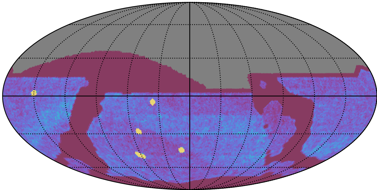
ddf_acor_sf10_lsf30_lsr10_v3.4_10yrs All sky all bands: NVisits
