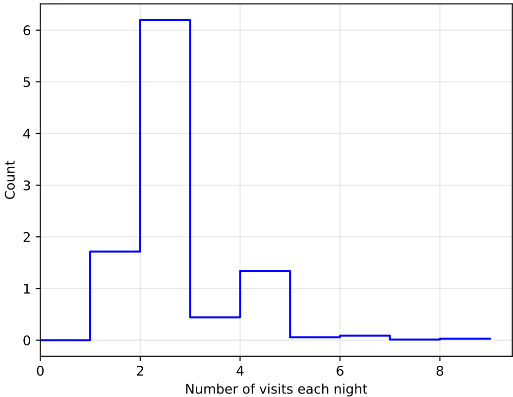
ddf_acor_sf10_lsf30_lsr10_v3.4_10yrs All sky: NVisitsPerNight 1e6
