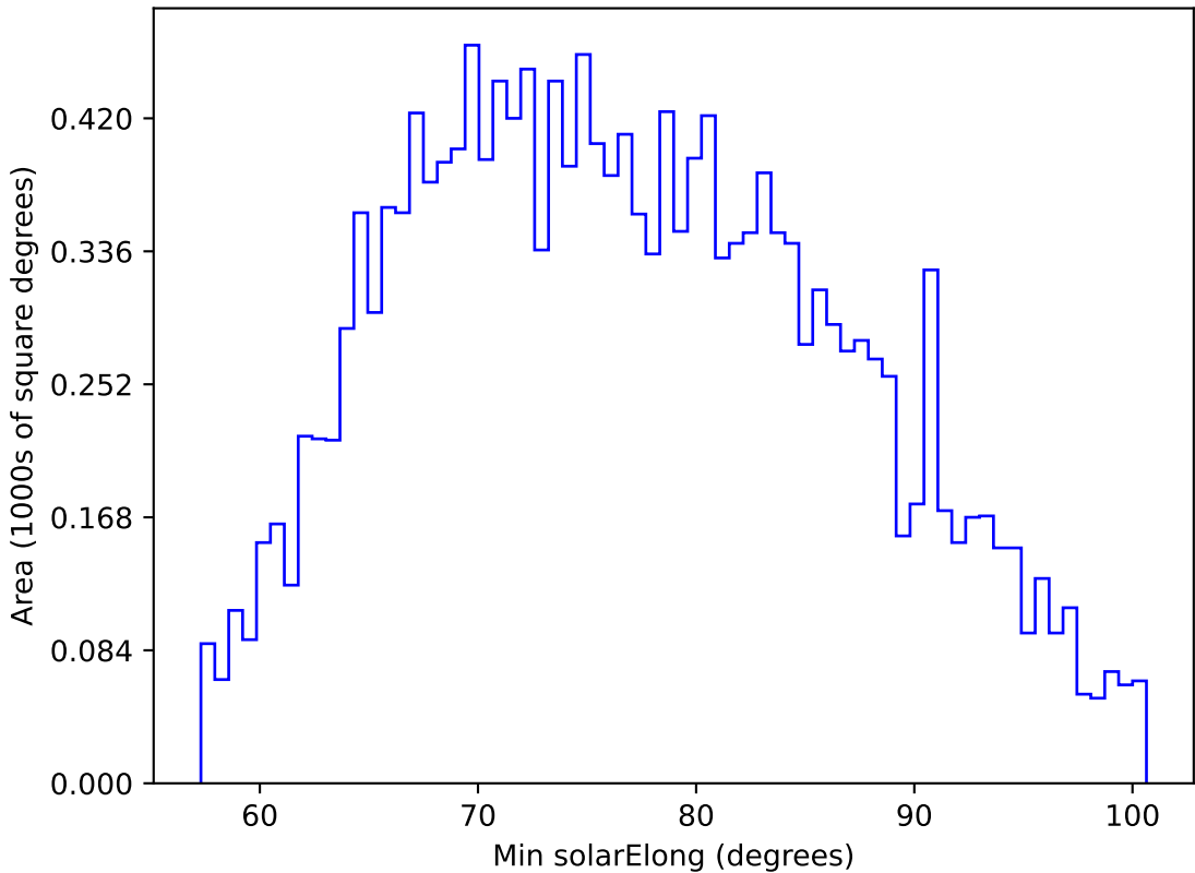
ddf_acor_sf10_lsf30_lsr10_v3.4_10yrs WFD u band: Min solarElong
