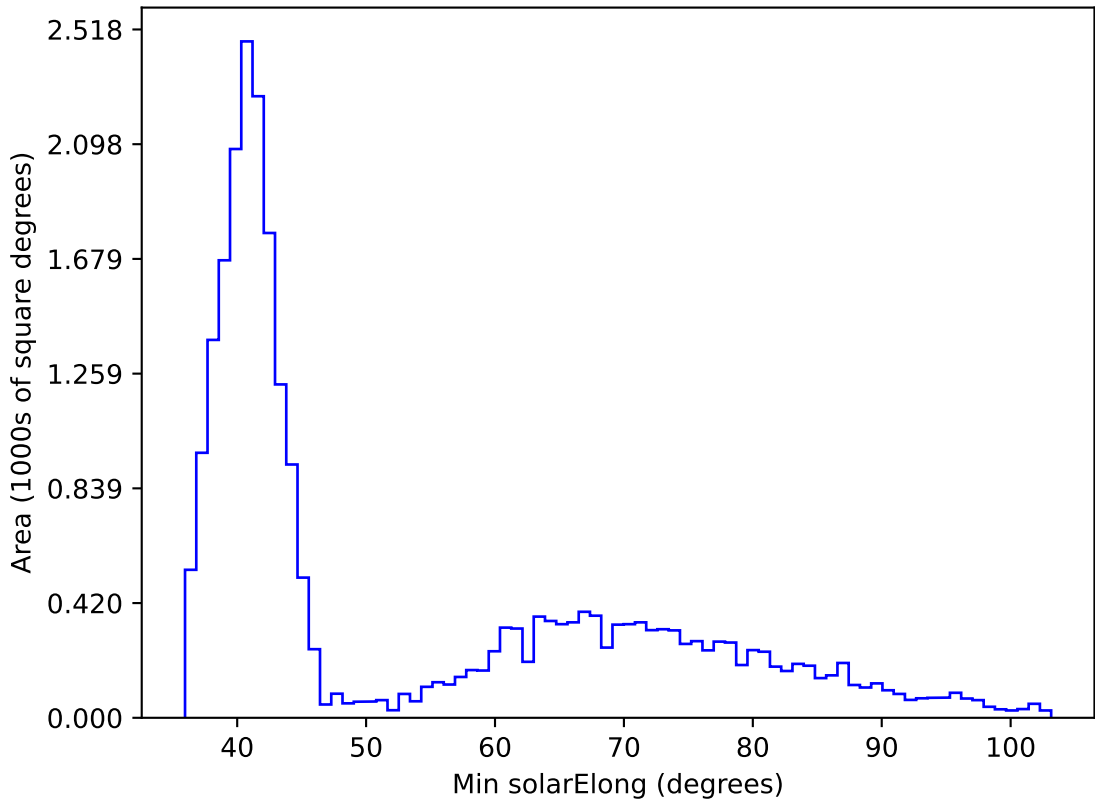
ddf_acor_sf10_lsf30_lsr10_v3.4_10yrs All sky z band: Min solarElong
