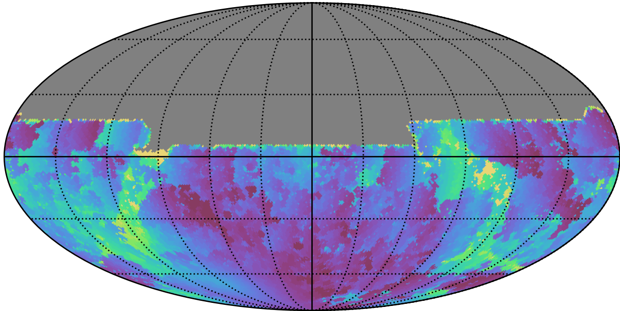
ddf_acor_sf10_lsf30_lsr10_v3.4_10yrs All sky u band: Min solarElong
