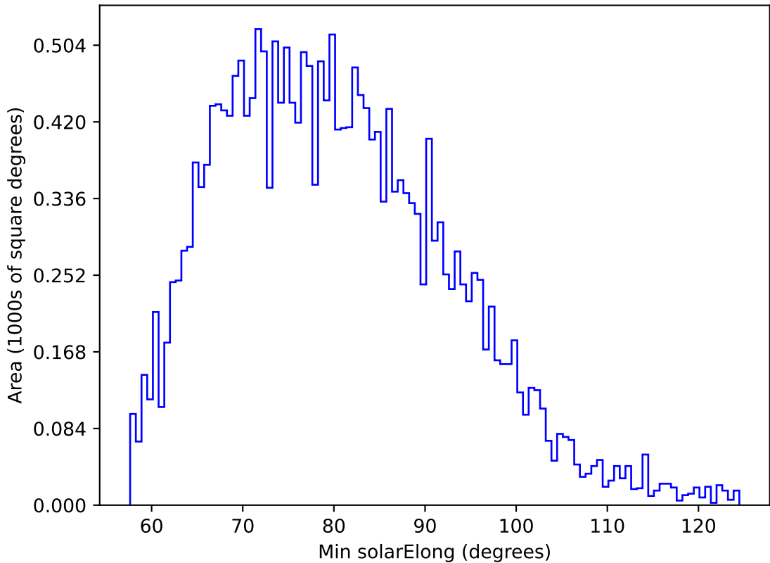
ddf_acor_sf10_lsf30_lsr10_v3.4_10yrs All sky u band: Min solarElong
