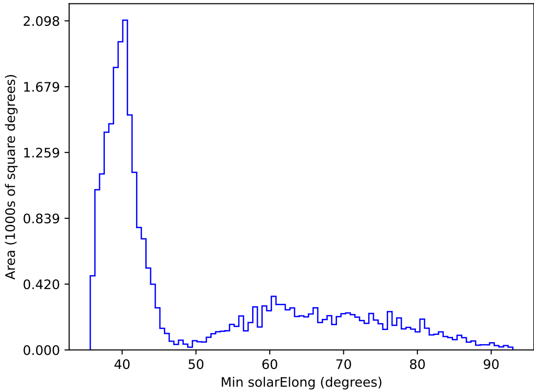
ddf_acor_sf10_lsf30_lsr10_v3.4_10yrs All sky all bands: Min solarElong
