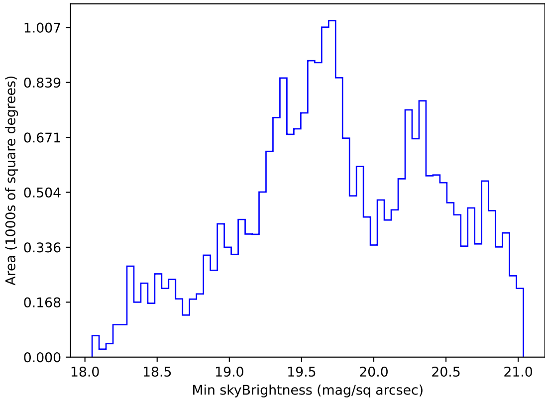
ddf_acor_sf10_lsf30_lsr10_v3.4_10yrs Yr 1 r band: Min skyBrightness
