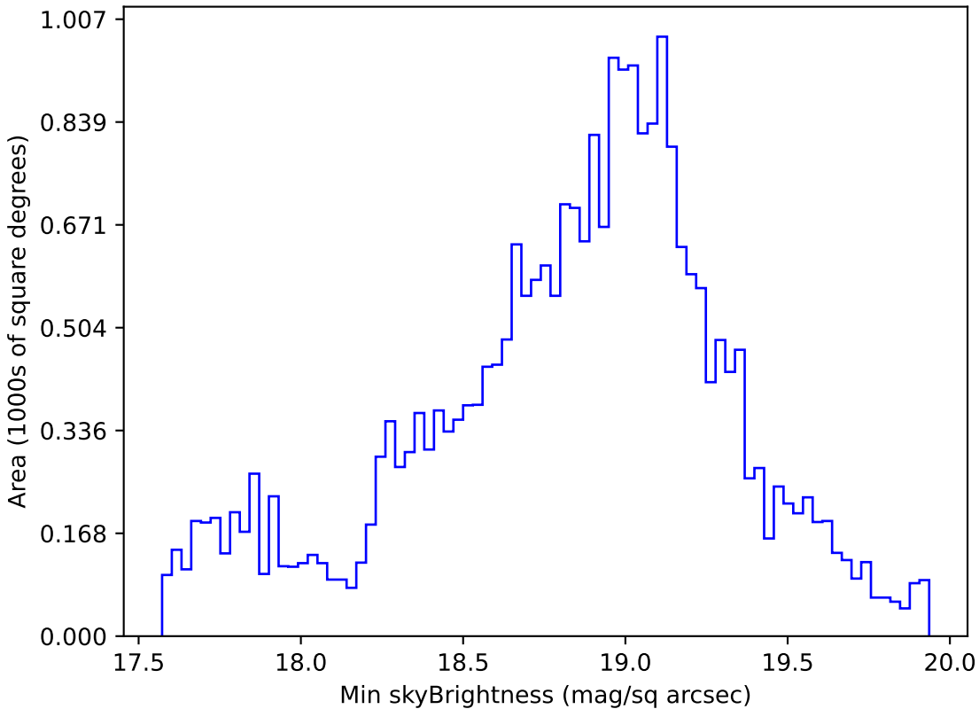
ddf_acor_sf10_lsf30_lsr10_v3.4_10yrs Yr 1 i band: Min skyBrightness
