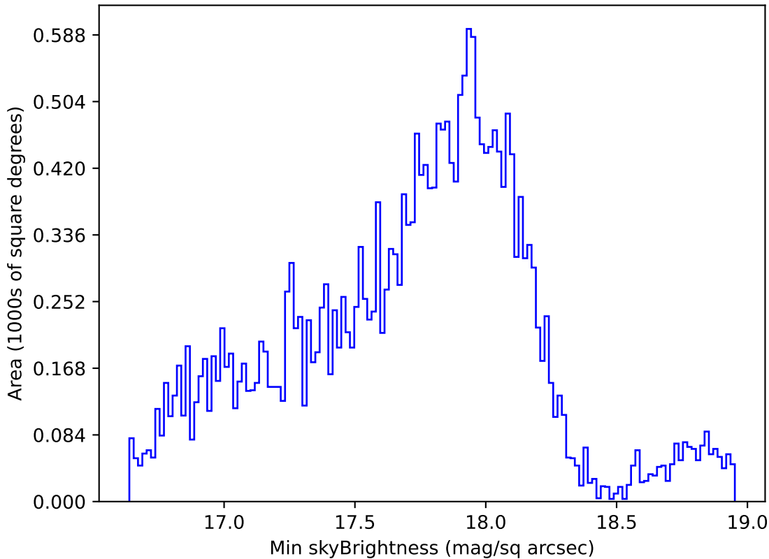
ddf_acor_sf10_lsf30_lsr10_v3.4_10yrs Yr 1 all bands: Min skyBrightness
