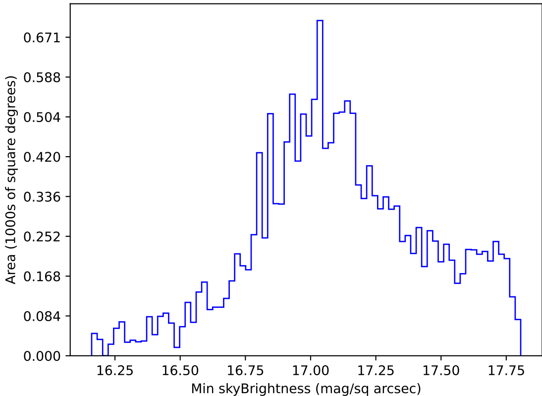
ddf_acor_sf10_lsf30_lsr10_v3.4_10yrs WFD y band: Min skyBrightness
