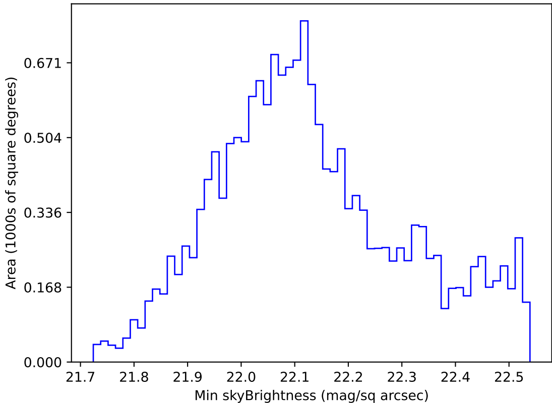
ddf_acor_sf10_lsf30_lsr10_v3.4_10yrs WFD u band: Min skyBrightness
