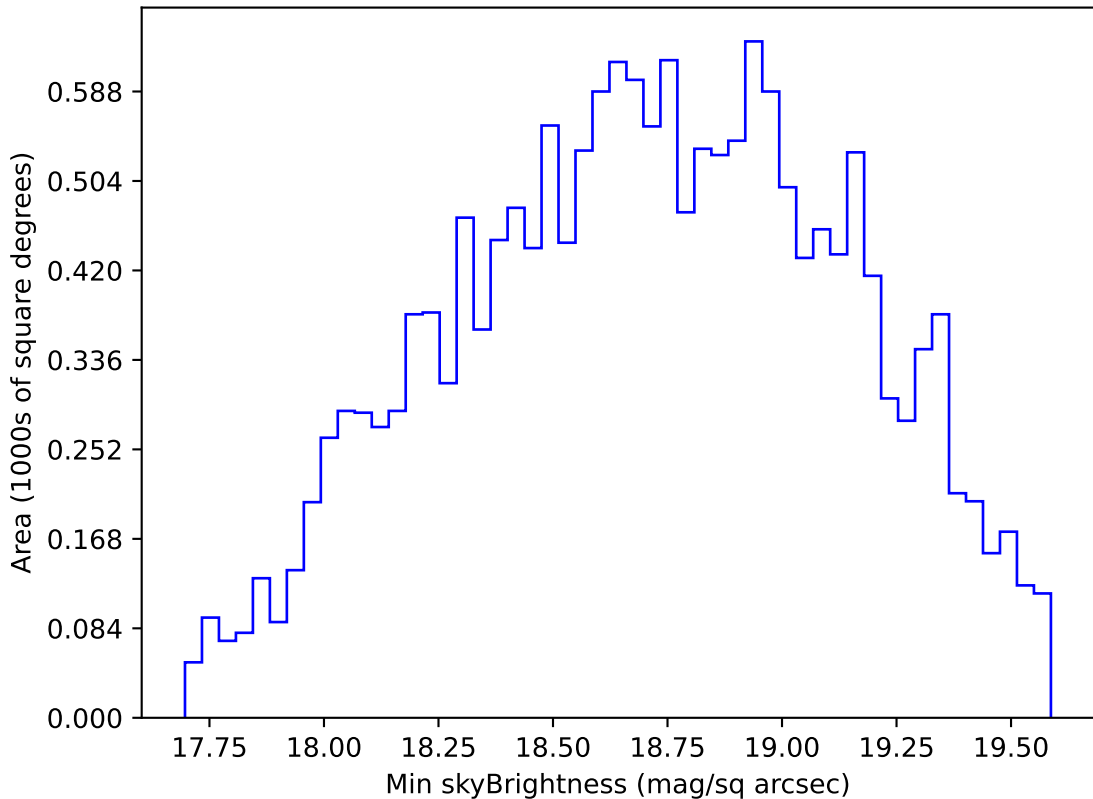
ddf_acor_sf10_lsf30_lsr10_v3.4_10yrs WFD r band: Min skyBrightness
