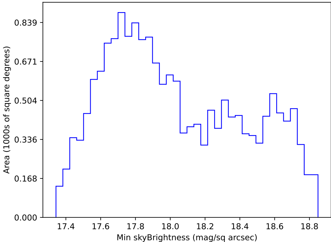
ddf_acor_sf10_lsf30_lsr10_v3.4_10yrs WFD i band: Min skyBrightness
