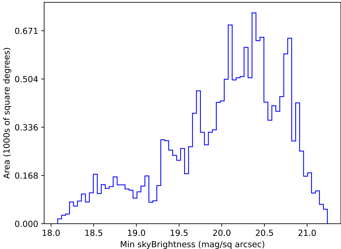
ddf_acor_sf10_lsf30_lsr10_v3.4_10yrs WFD g band: Min skyBrightness
