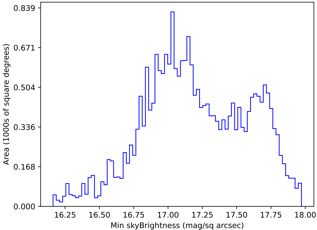
ddf_acor_sf10_lsf30_lsr10_v3.4_10yrs All sky y band: Min skyBrightness
